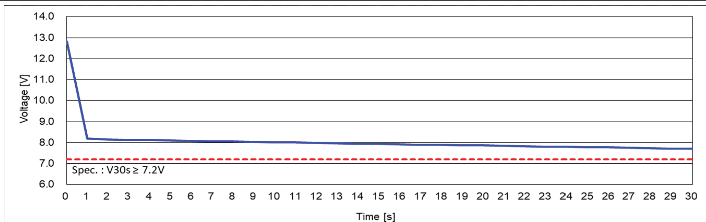
Cold Cranking Test Graph (-18°C, Icc 750A)
